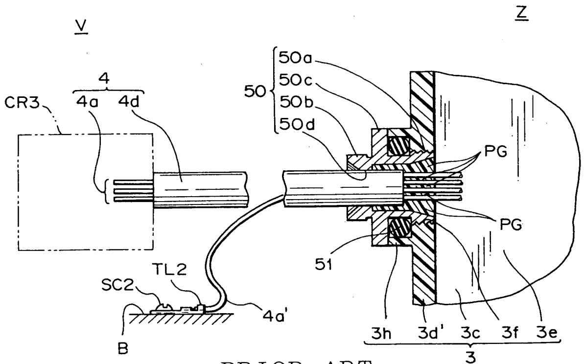
PRIOR ART FIG. 13
